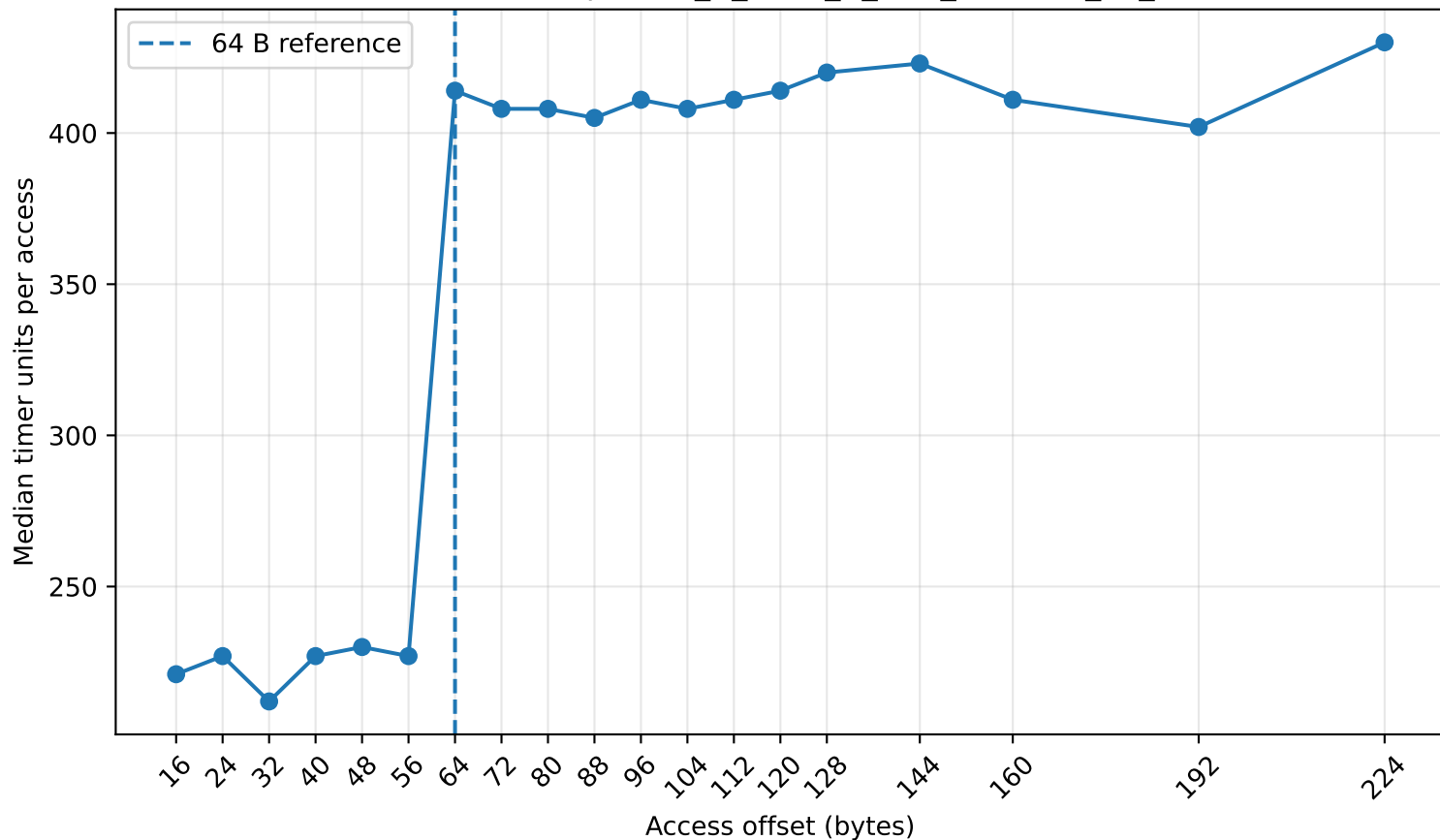
Hazel line-size sweep: Intel_R_Xeon_R_CPU_E5-2650_v3_2.30GHz
