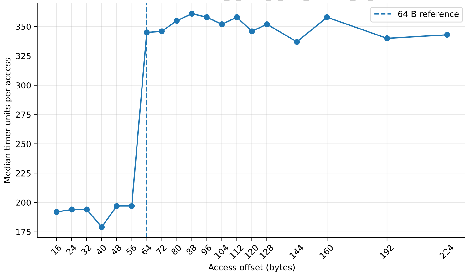
Hazel line-size sweep: Intel_R_Xeon_R_CPU_E5-2650_v4_2.20GHz
