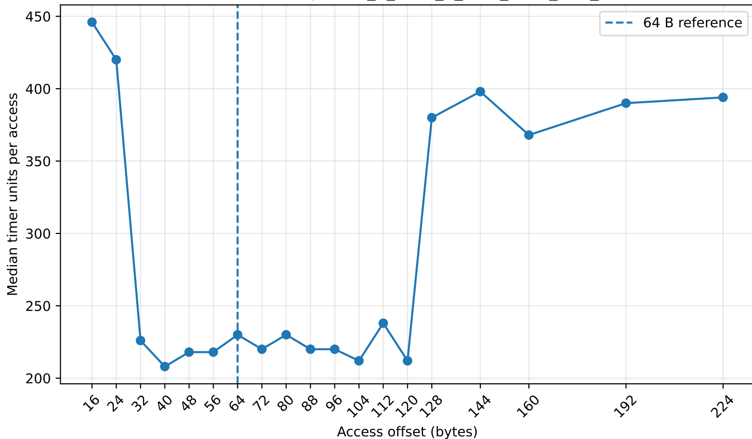
Hazel line-size sweep: Intel_R_Xeon_R_Gold_6326_CPU_2.90GHz
