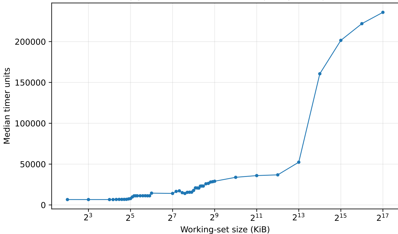
Upgrade — Phase-I cache capacity sweep
