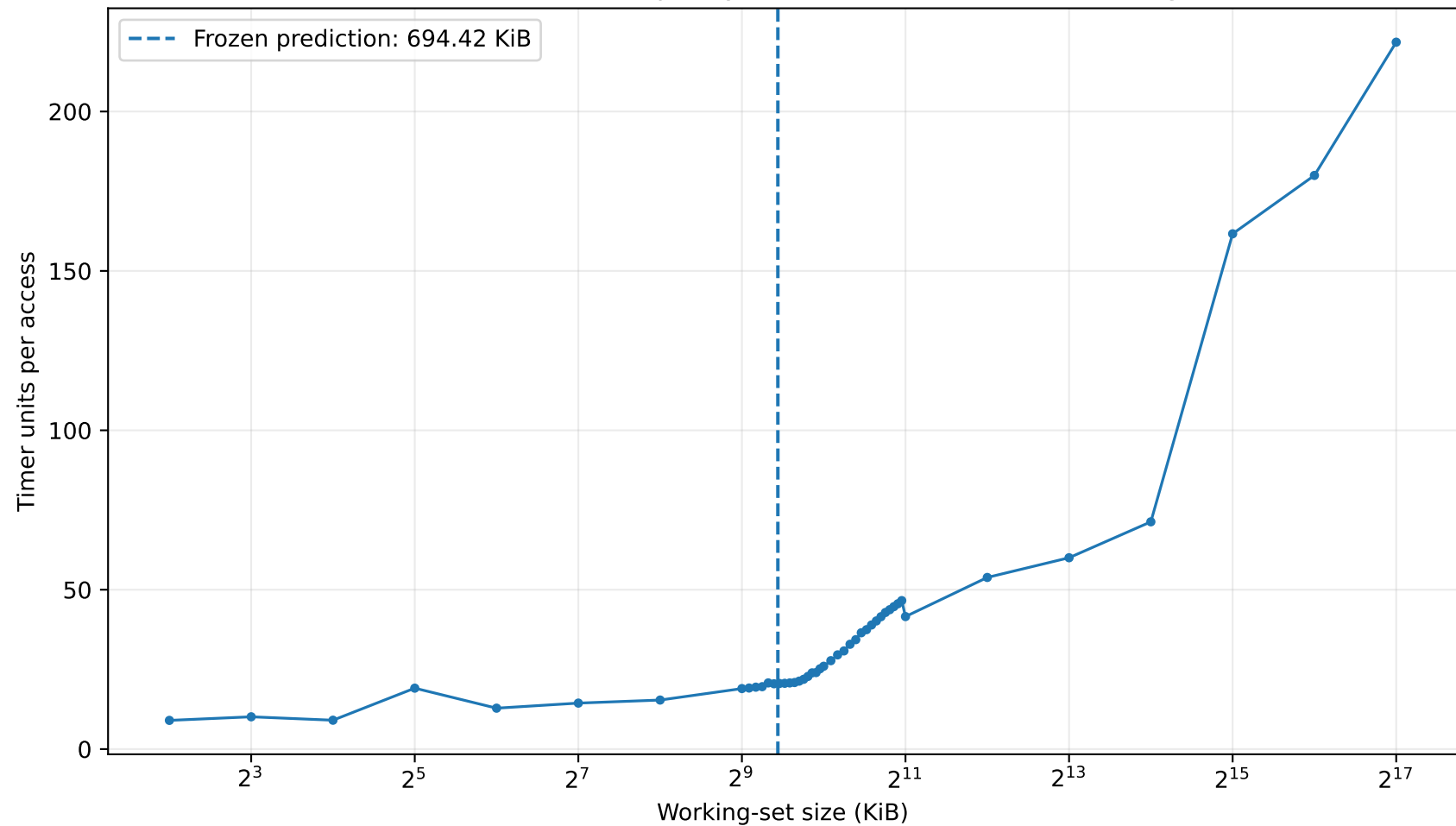
Hazel: Frozen L2 Capacity Prediction vs. Measured Timing
