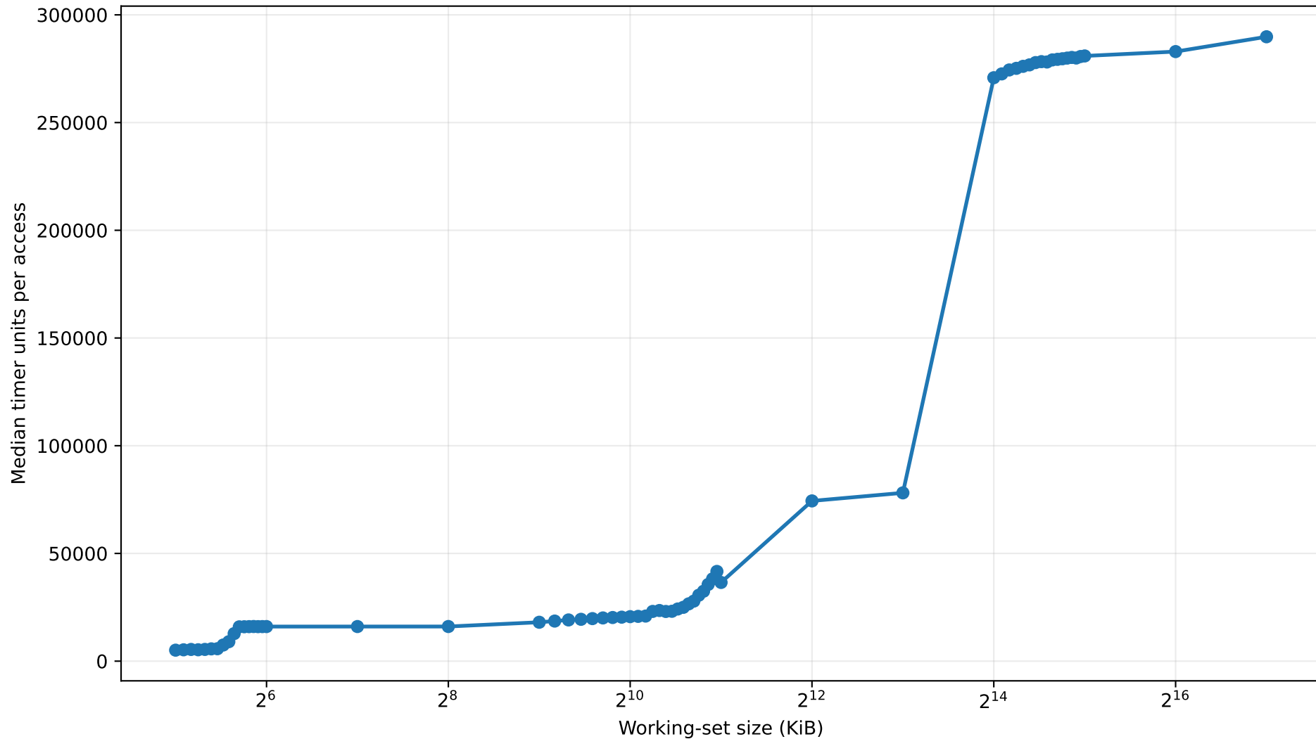
Artemisia — Cache latency experiment
