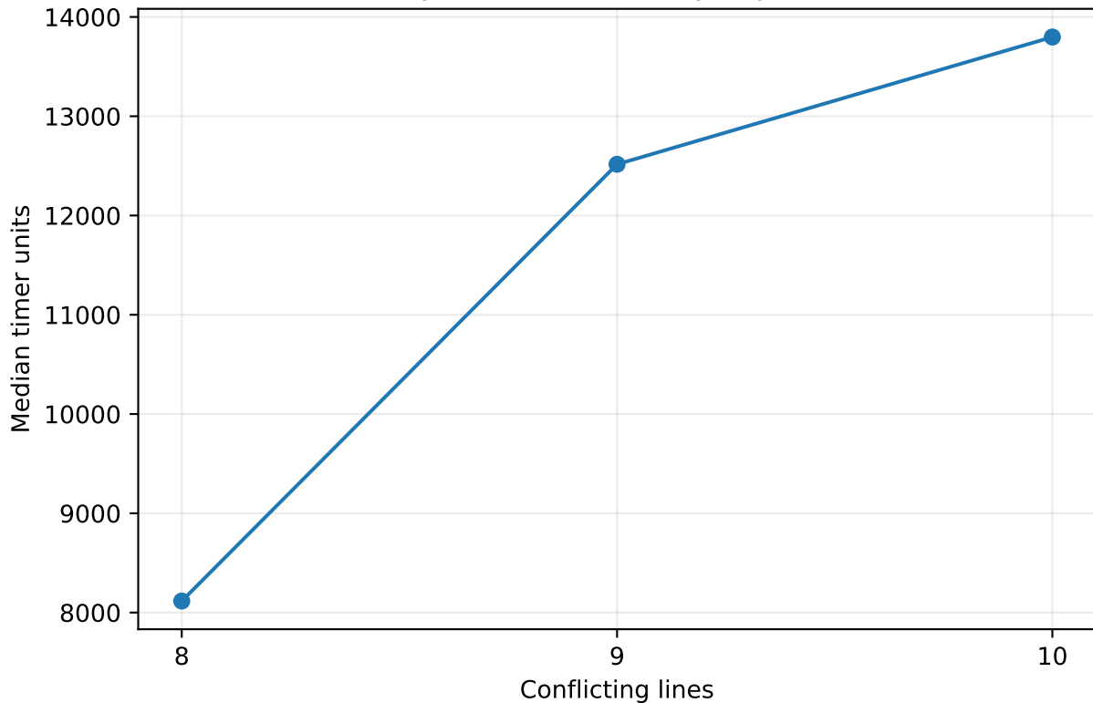
Ookay — L1 associativity experiment
