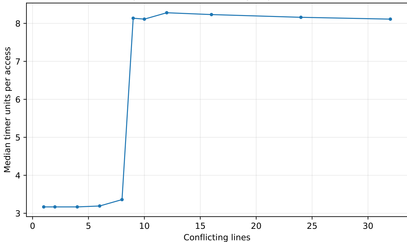
Skylark — L1 associativity experiment
