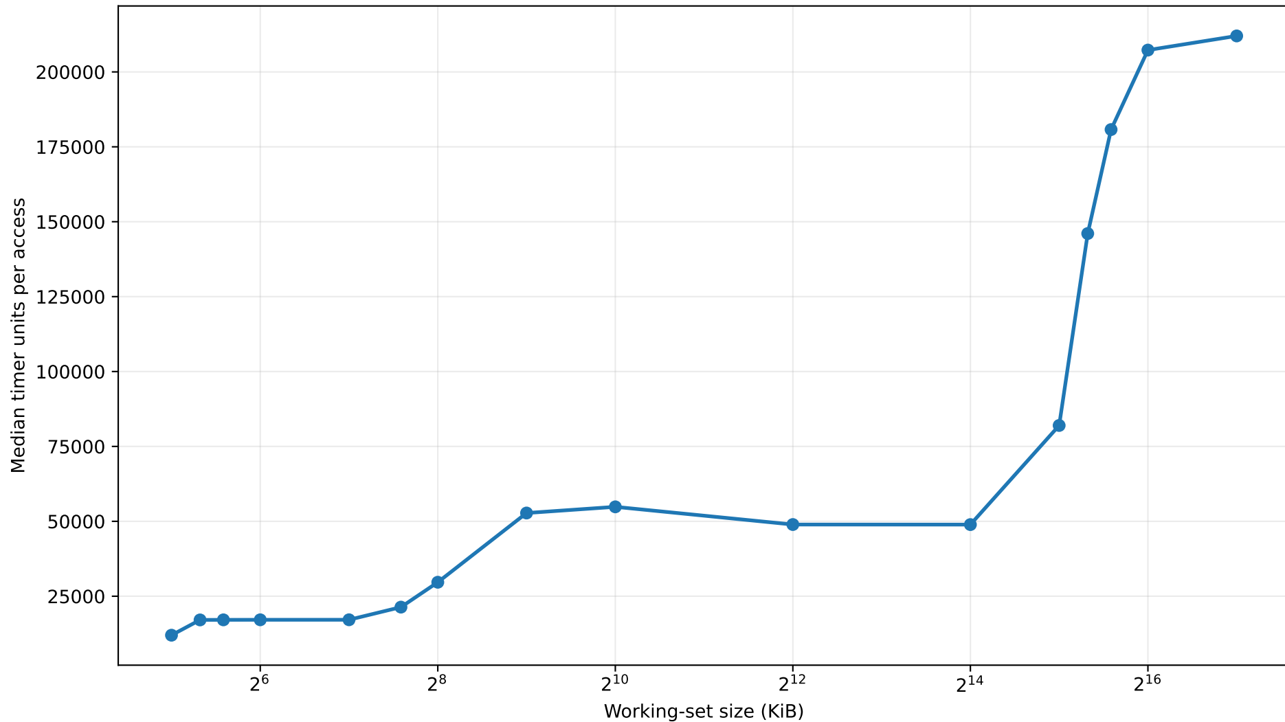
Sunbird — Cache latency experiment
