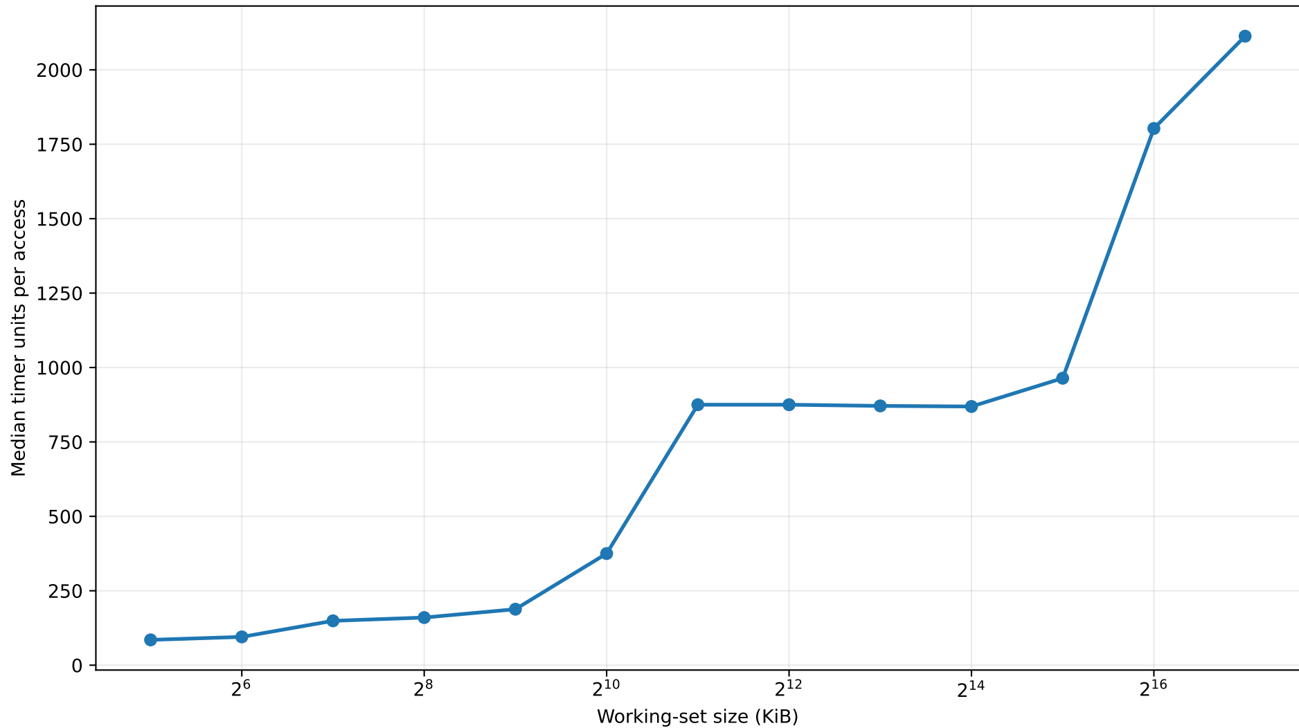
Thunderbird — Cache latency experiment
