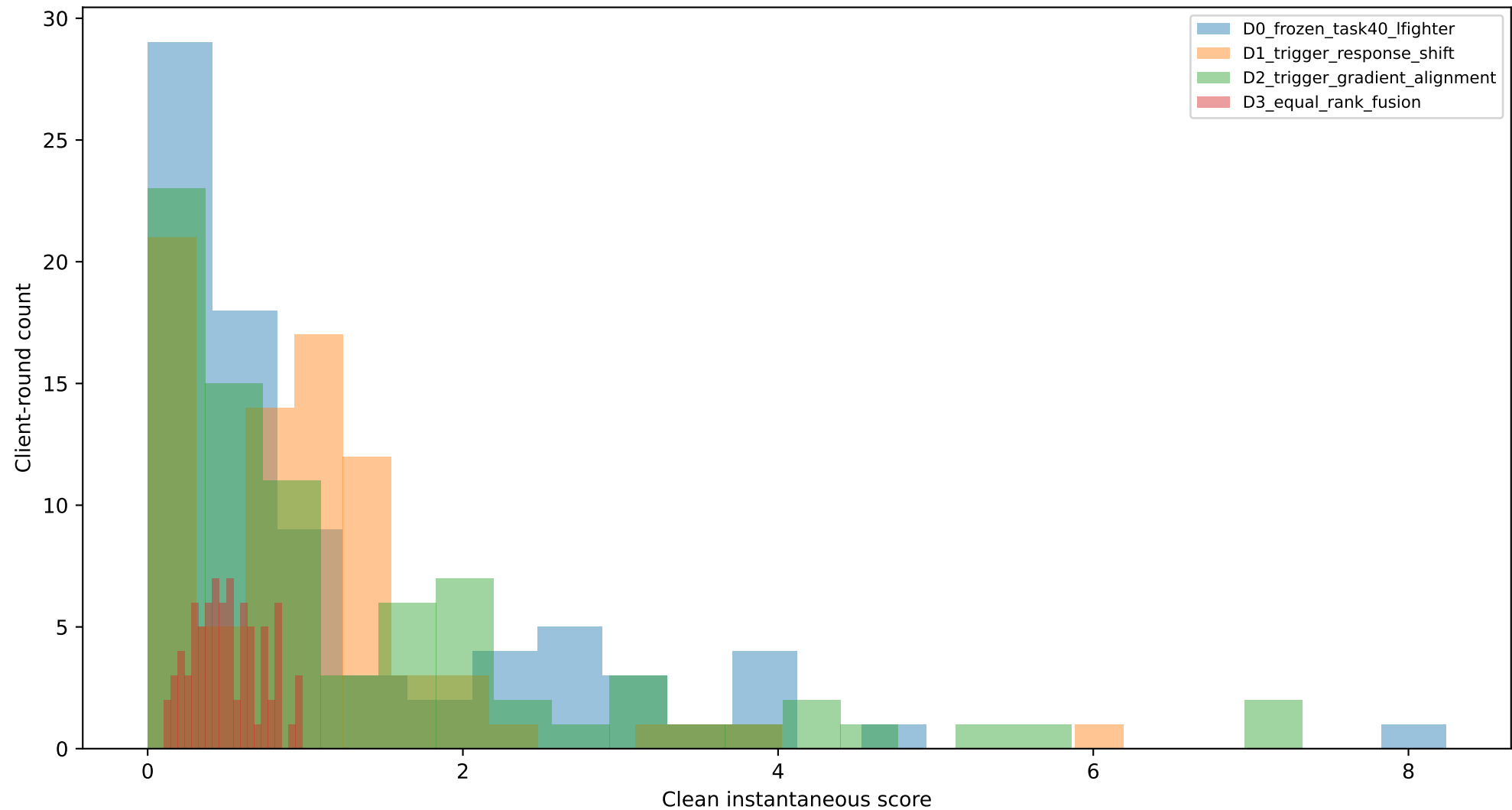
Task 41C clean score distributions, seed 123
