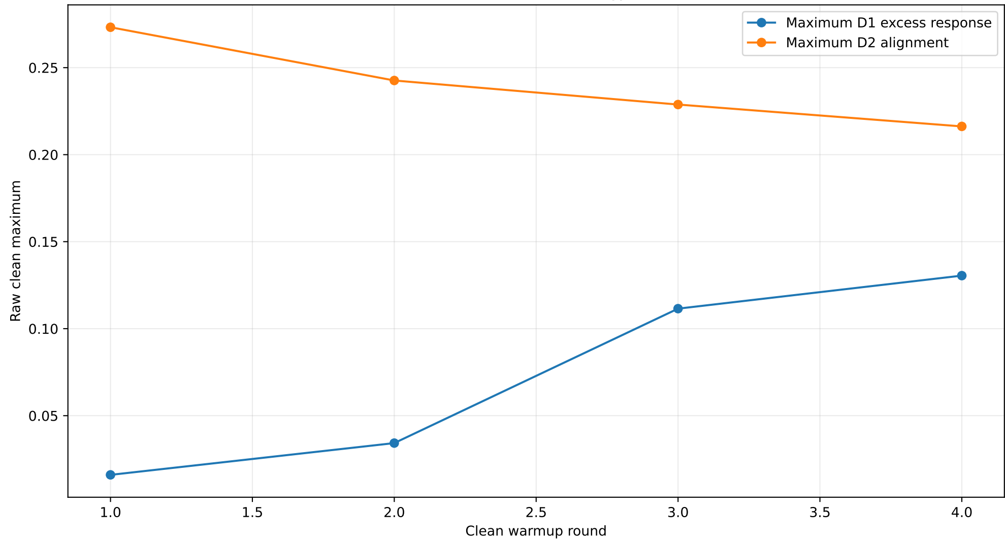
Task 41C clean feature chronology, seed 2026
