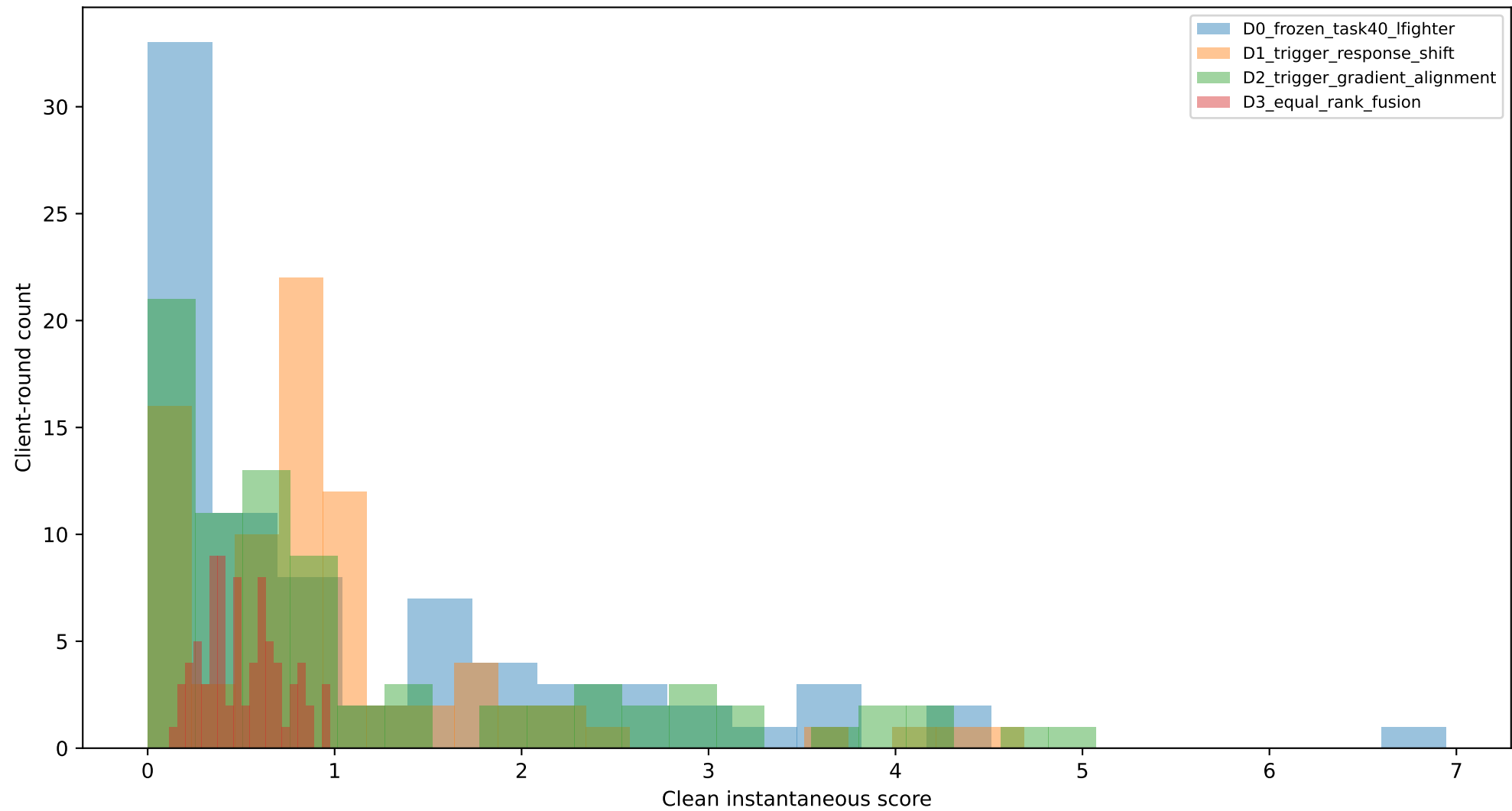
Task 41C clean score distributions, seed 2026
