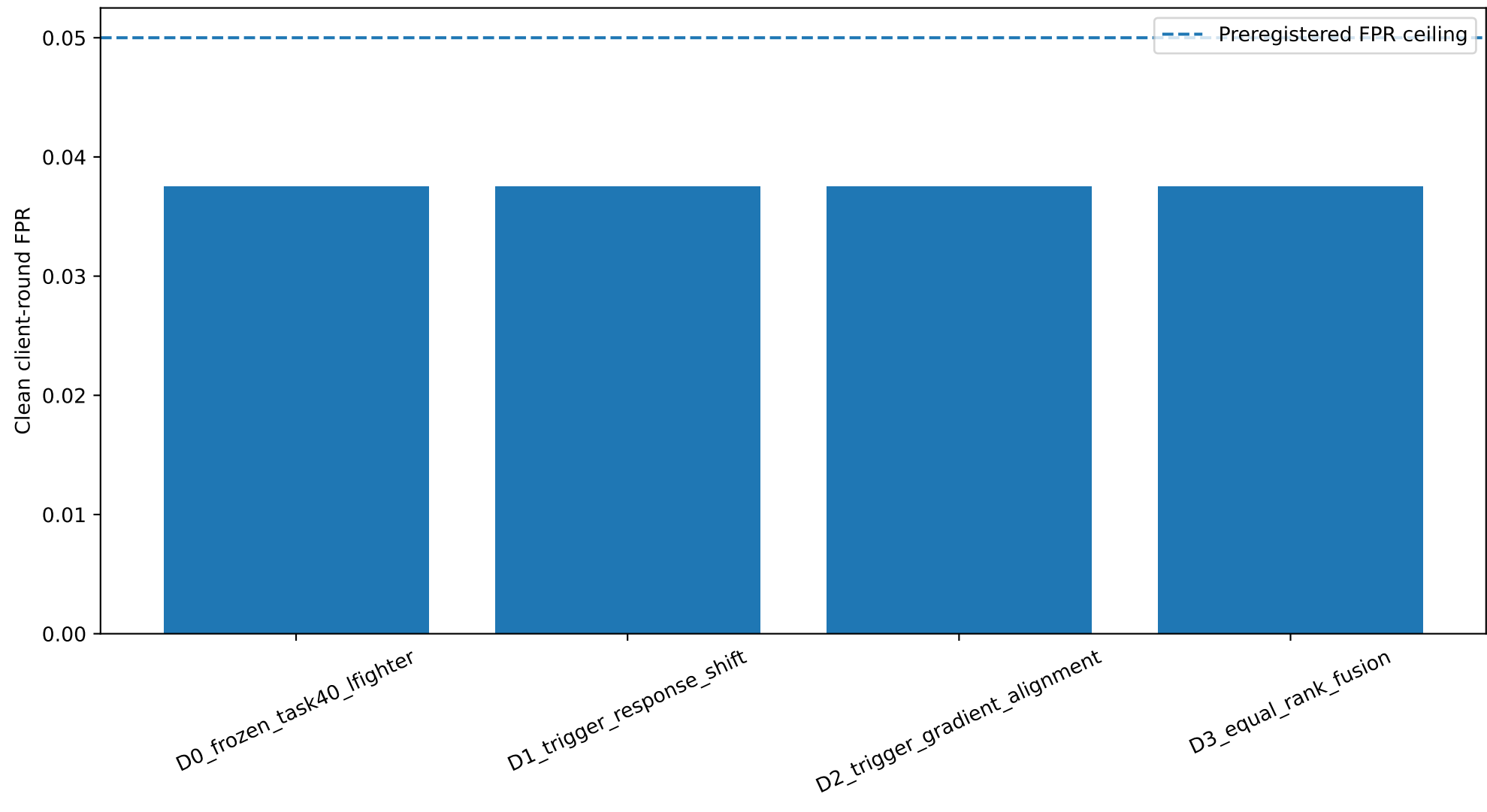
Task 41C clean detector FPR, seed 7
