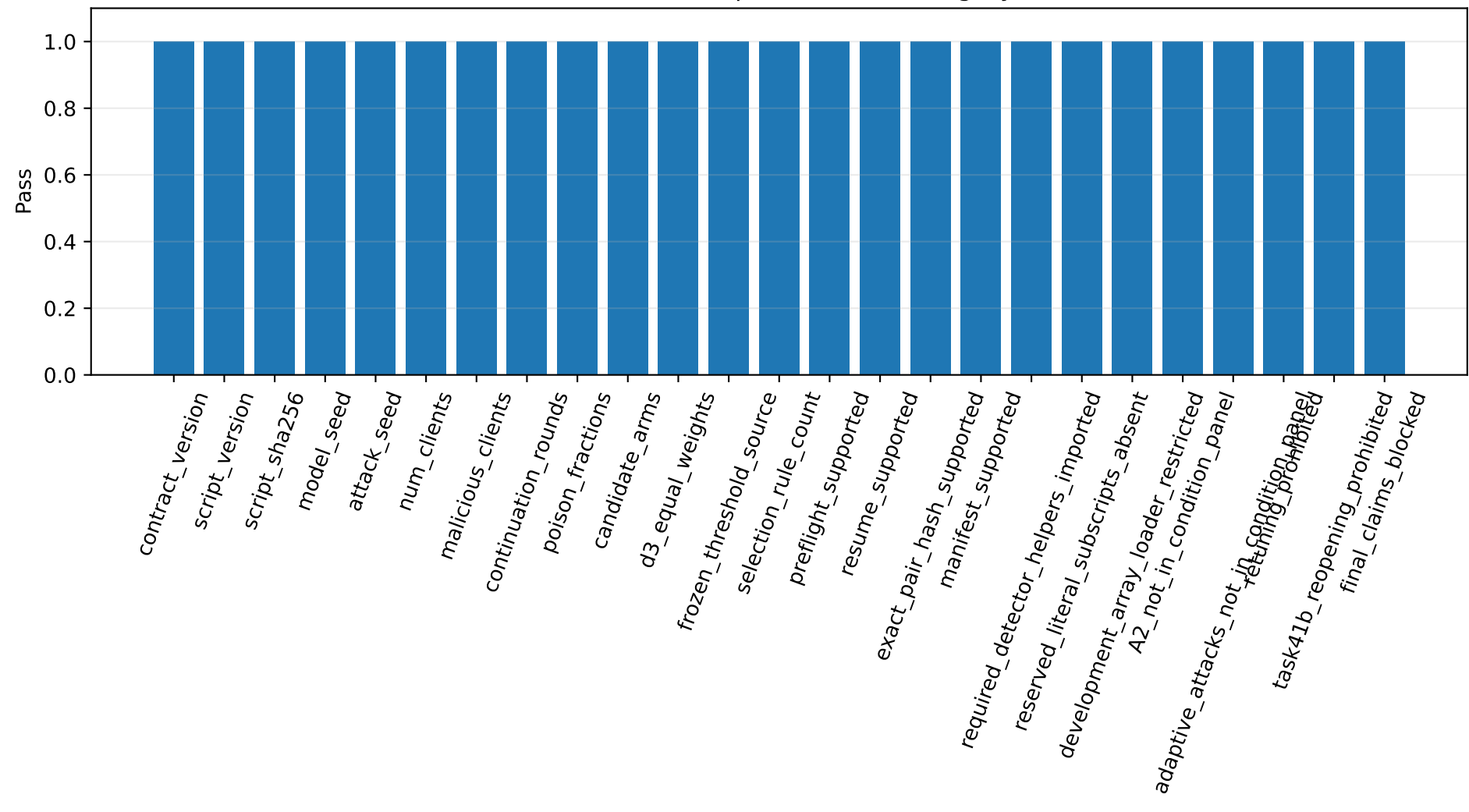
Task 41C C2 implementation integrity
