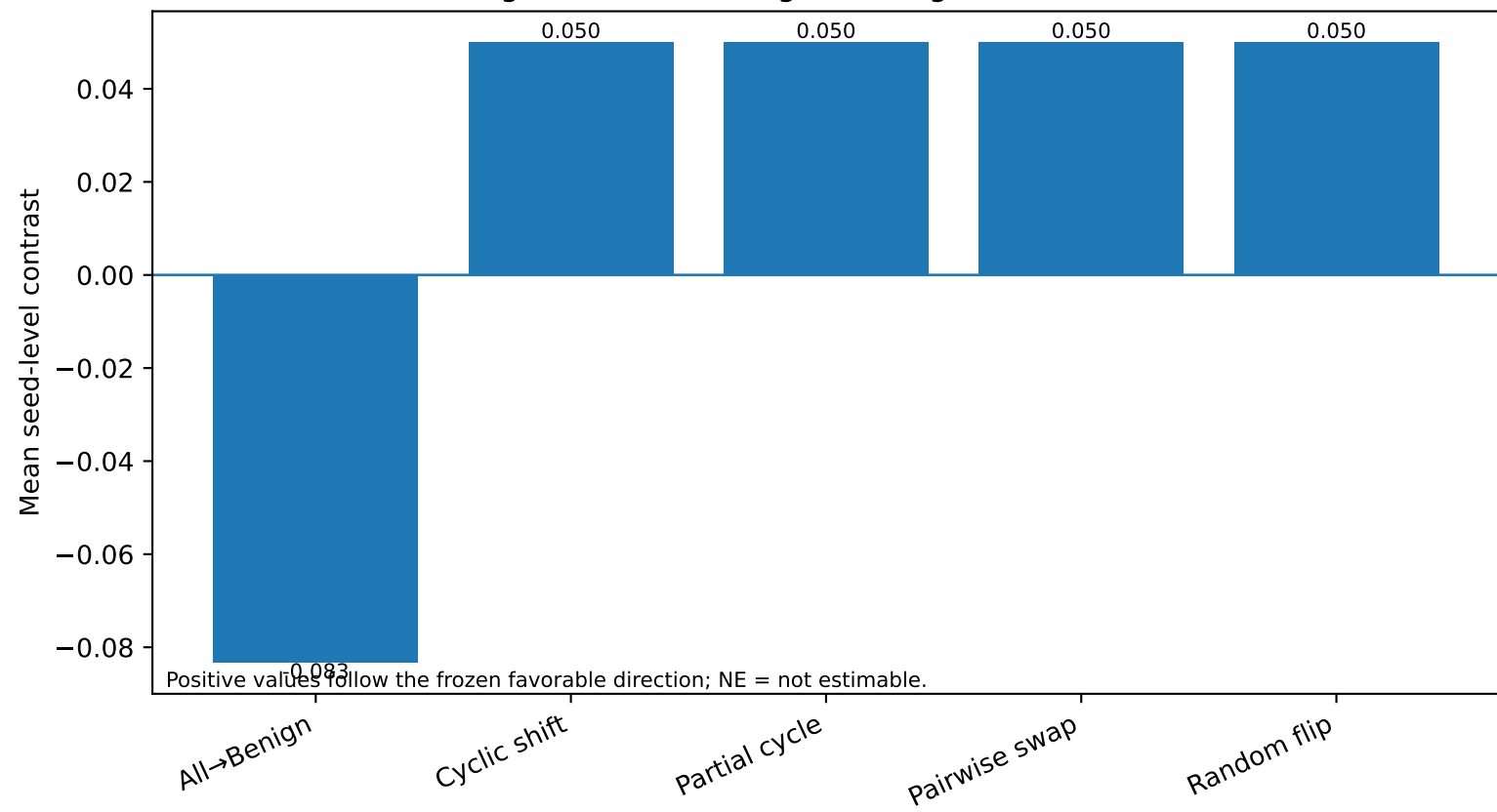
Benign-client FPR margin — Diagnostic — Round 8
