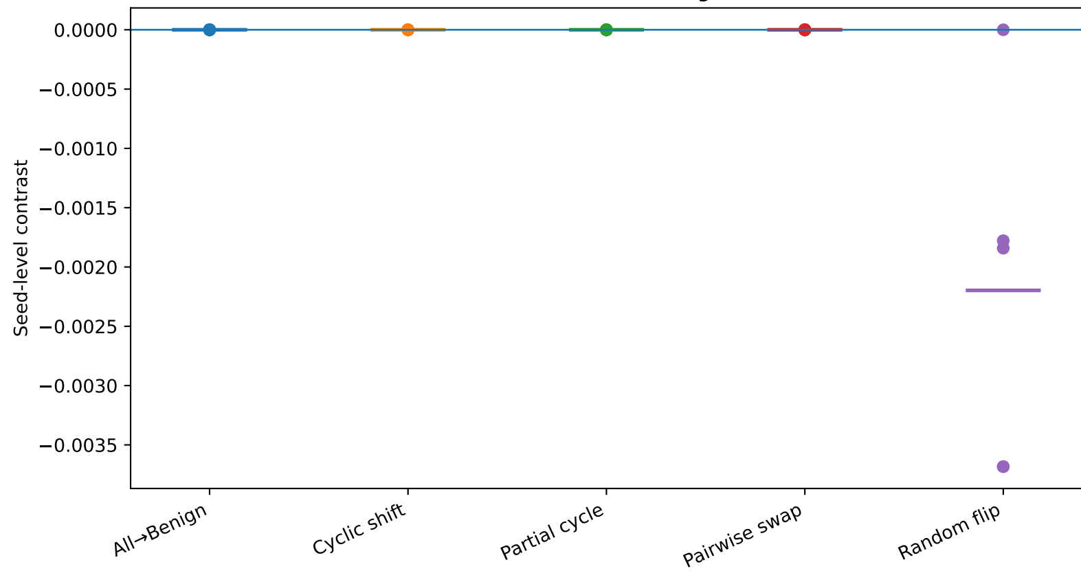
Seed-level Worst-class recall — Diagnostic — Round 8
