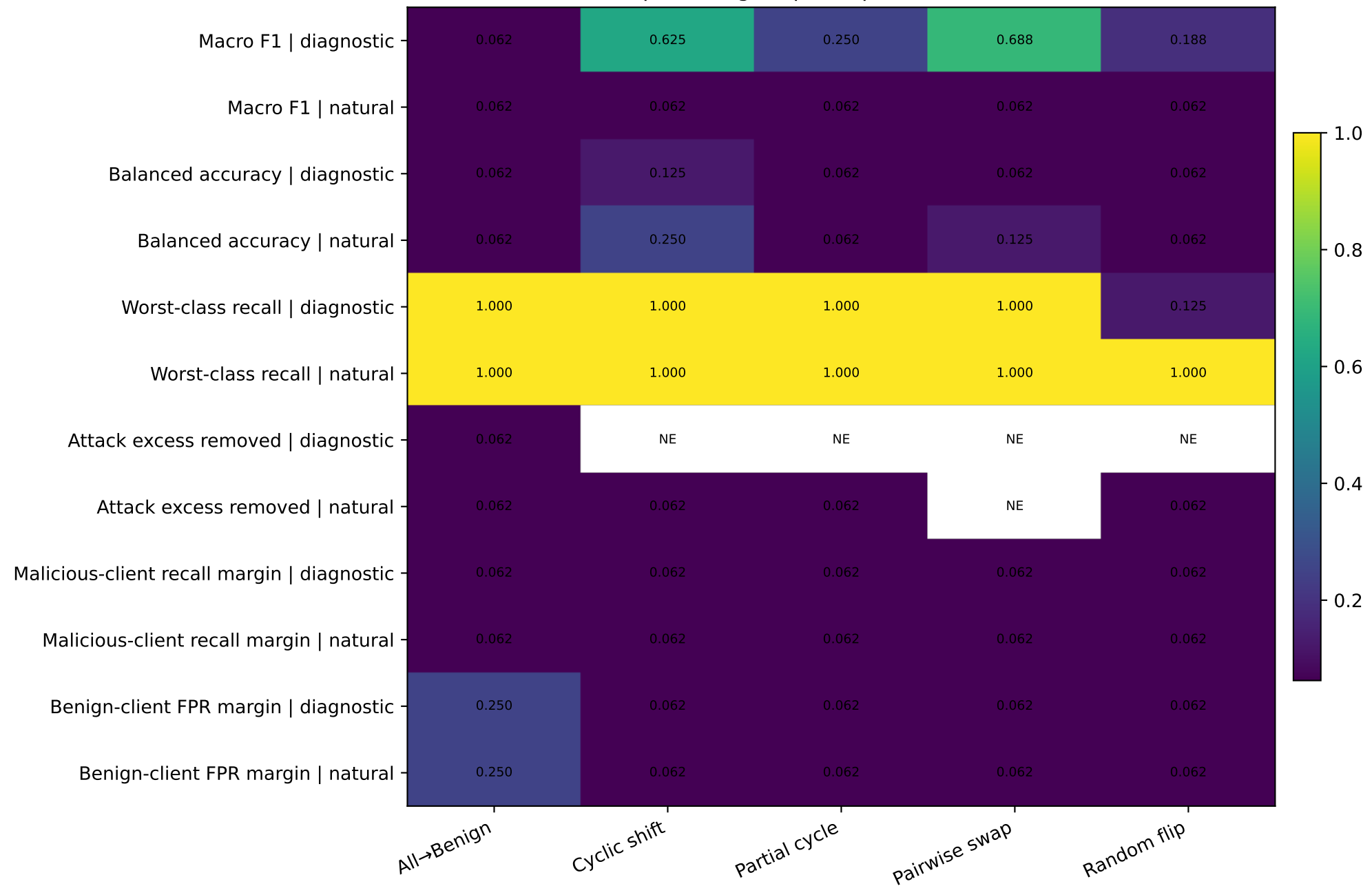
Exact paired sign-flip raw p-values (NE retained)
