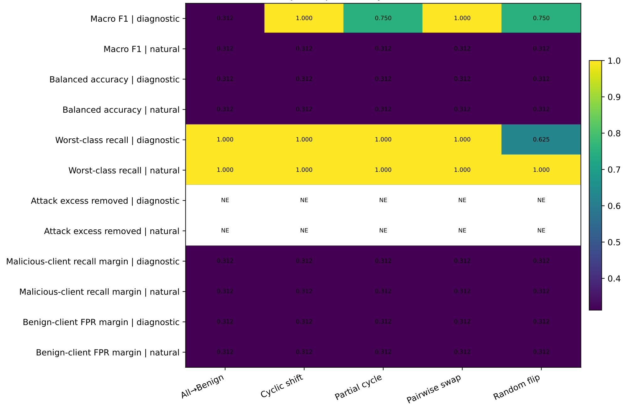
Holm-adjusted p-values by metric × dataset × attack
