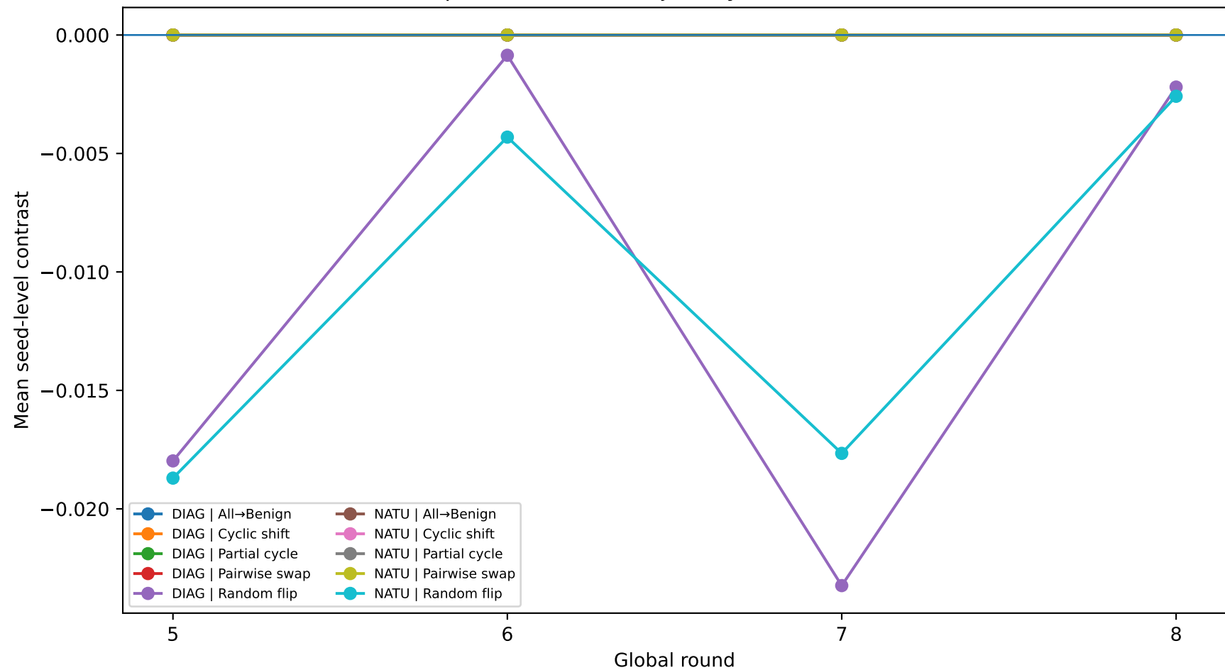
Descriptive round 5-8 trajectory — Worst-class recall
