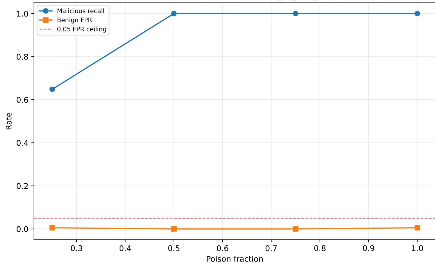
Task 44: D0 strength response, all_to_one_benign
