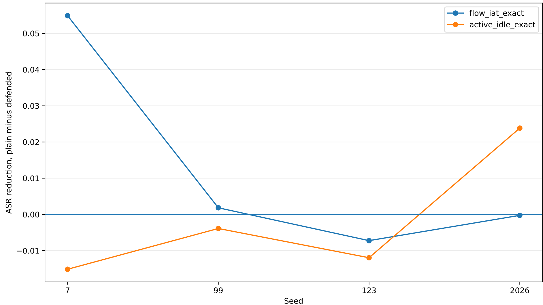
Task 41B seed-wise frozen-defense effect
