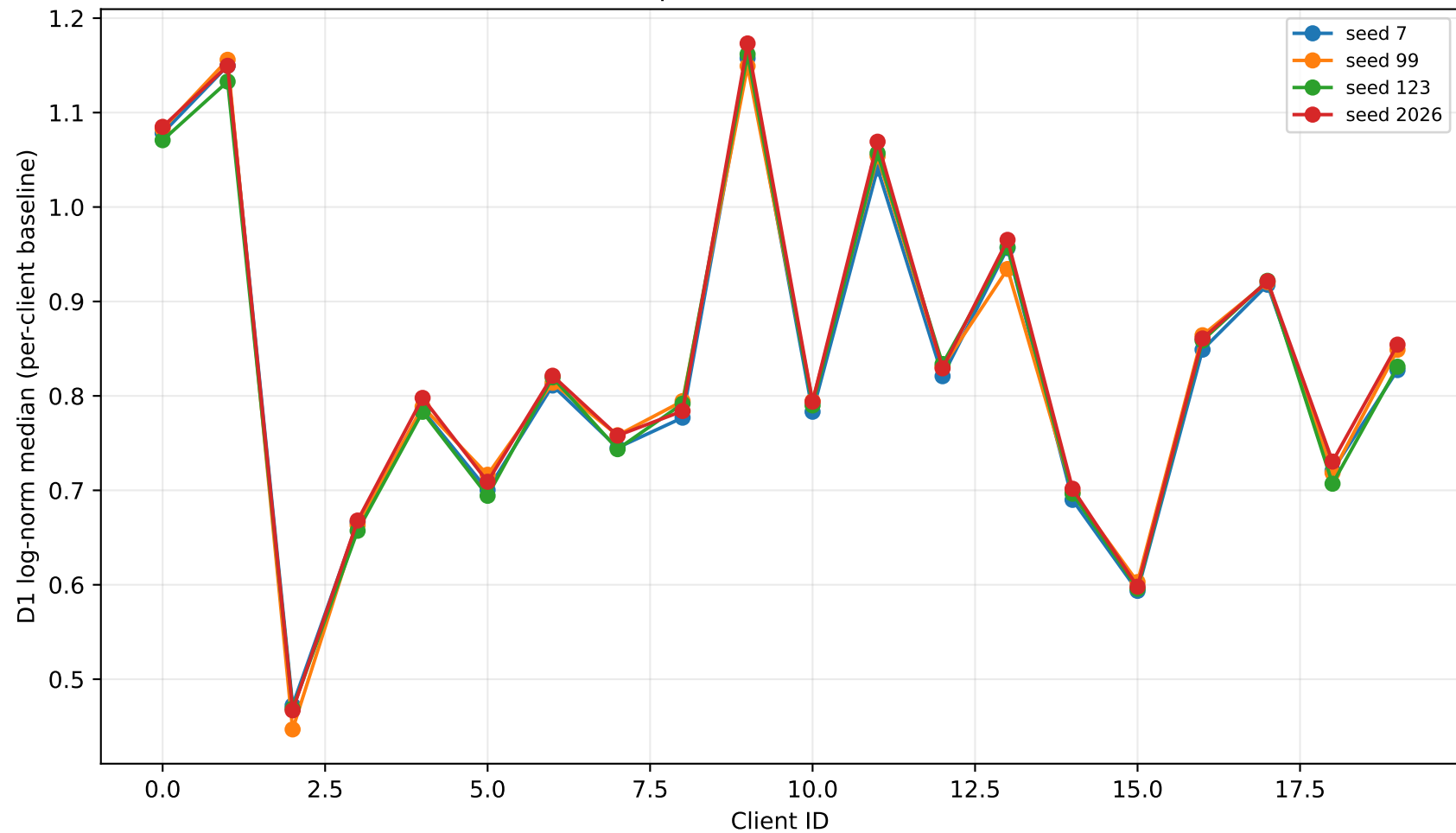
Task 42 C1a: D1 per-client norm baseline, all seeds
