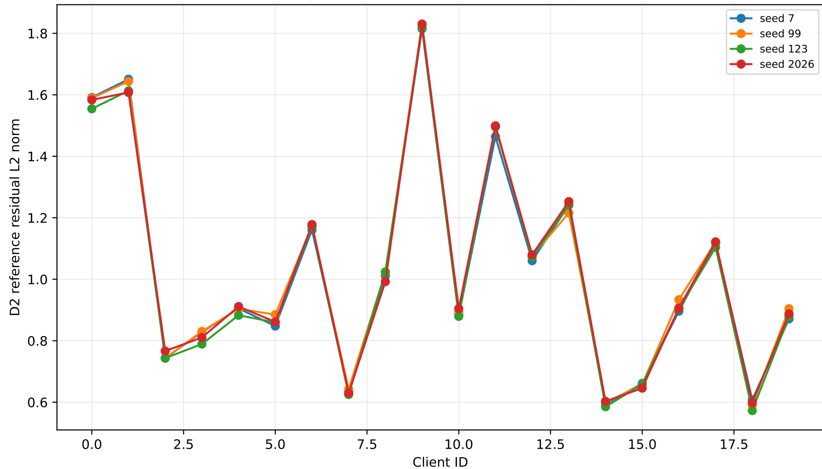
Task 42 C1a: D2 per-client reference-direction magnitude, all seeds
