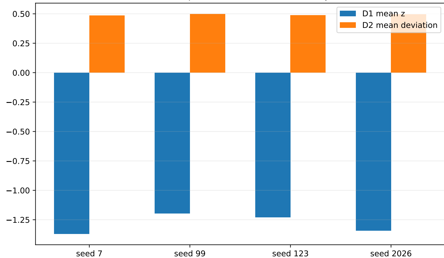
Task 42 C1b: pooled clean D1/D2 scores by seed
