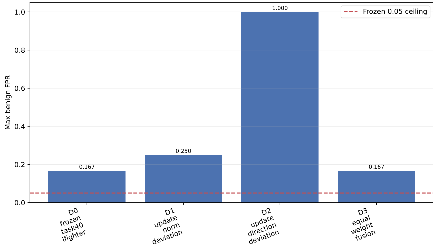
Task 42 C2: maximum benign FPR by candidate
