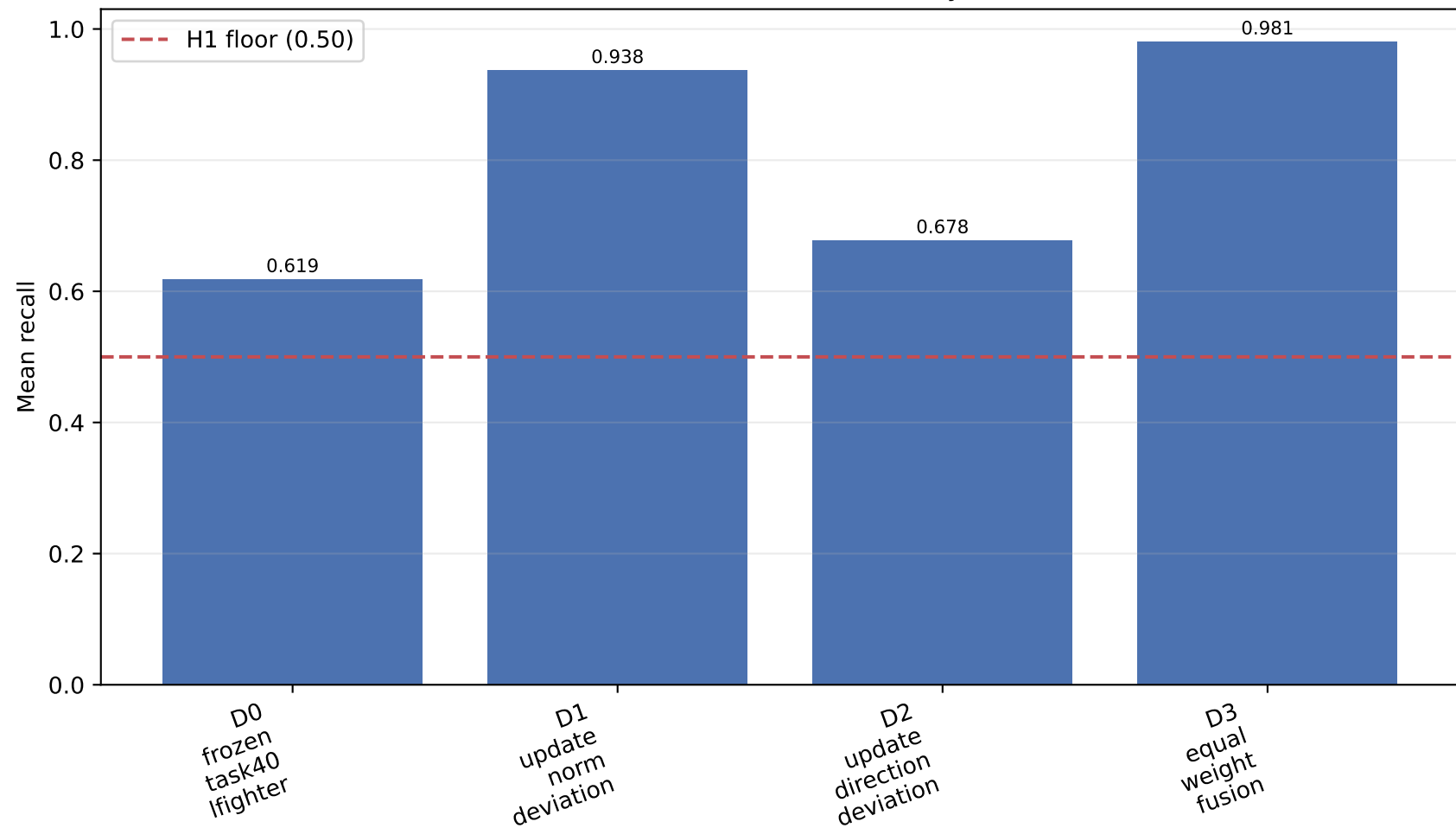
Task 42 C2: mean malicious recall by candidate
