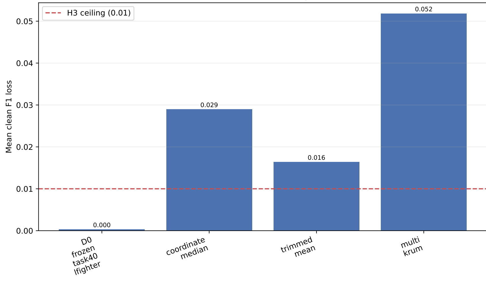
Task 43 C2: mean clean macro-F1 loss by arm (incl. baselines)
