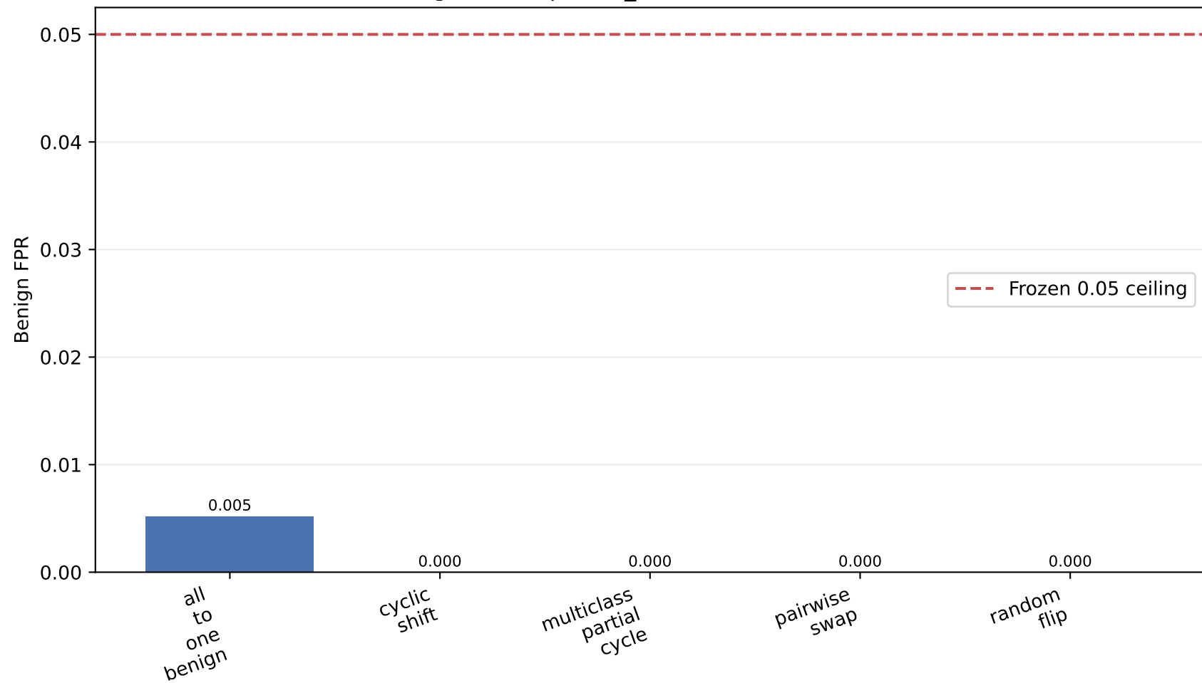
Task 44 C1: benign FPR at poison_fraction=1.0 (frozen Task 40 anchor)
