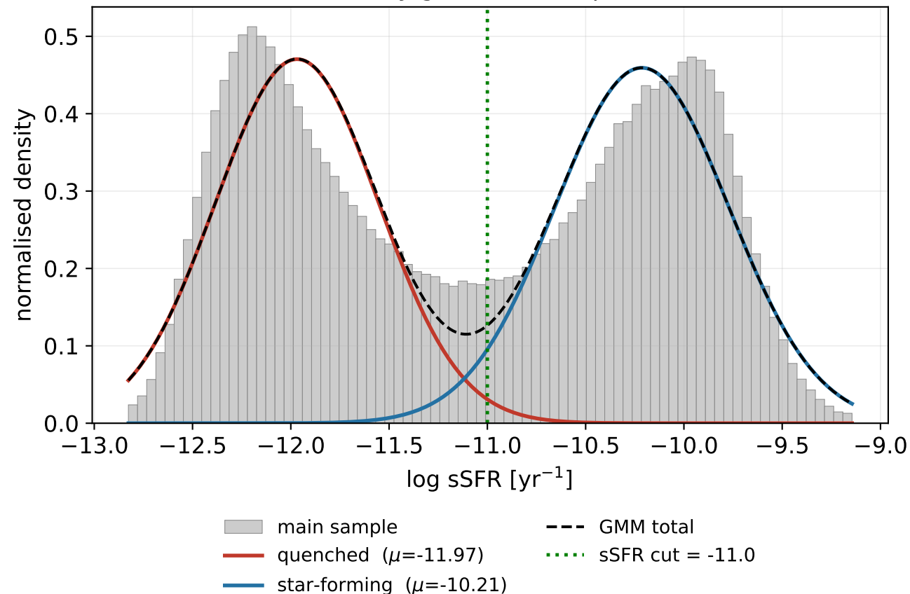
sSFR bimodality gate: PASS ( \Delta\mu = 1.75 dex)
