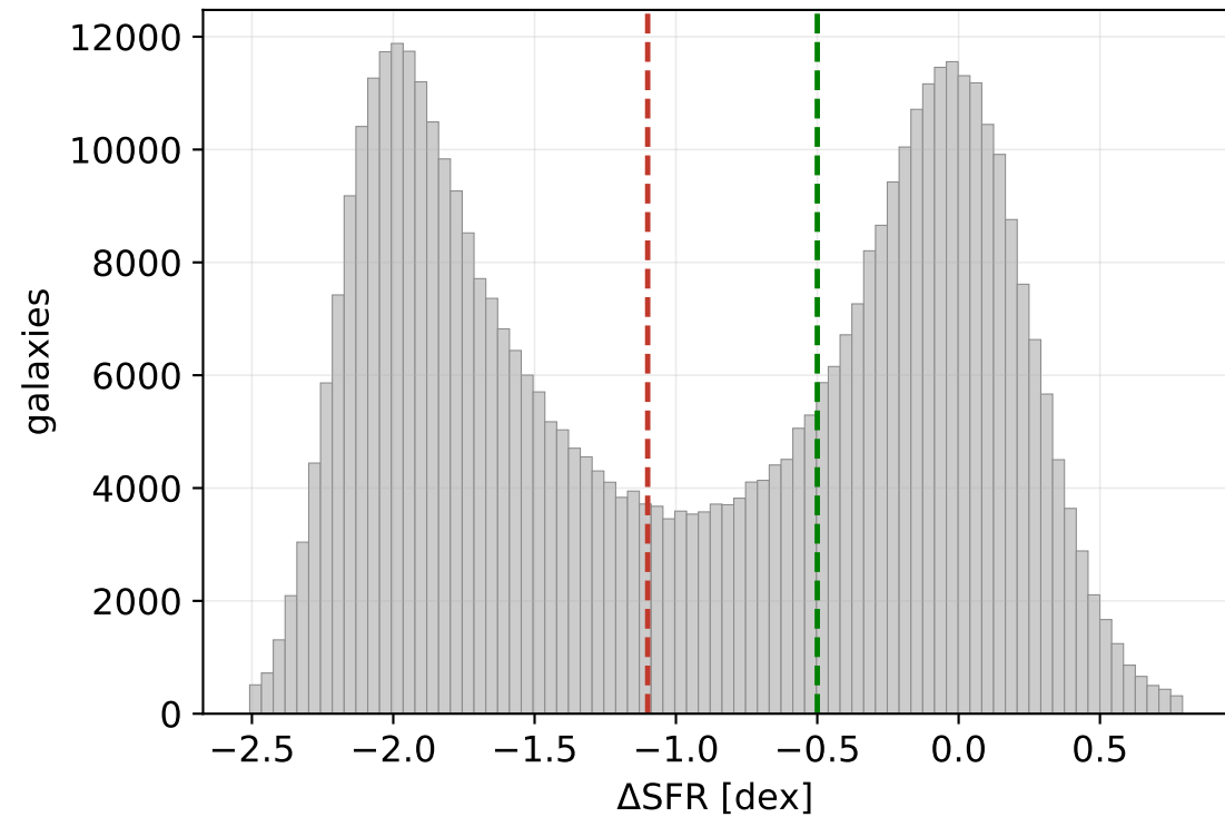
\Delta\text{SFR} distribution
