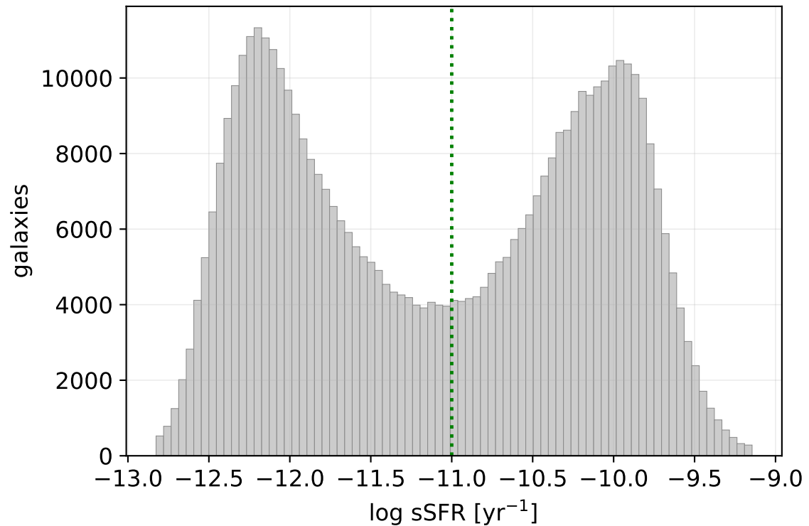
sSFR distribution (robustness cut)
