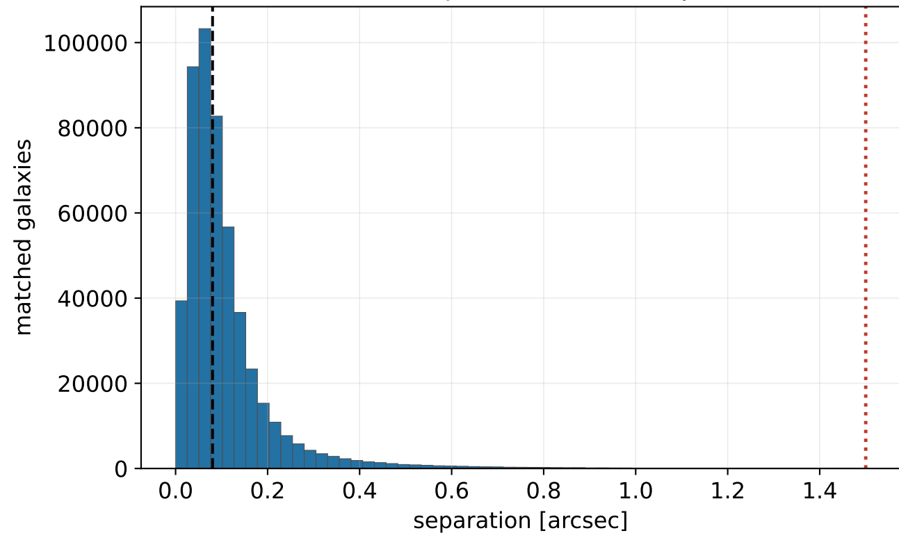
GZ DESI x MPA-JHU cross-match separation
