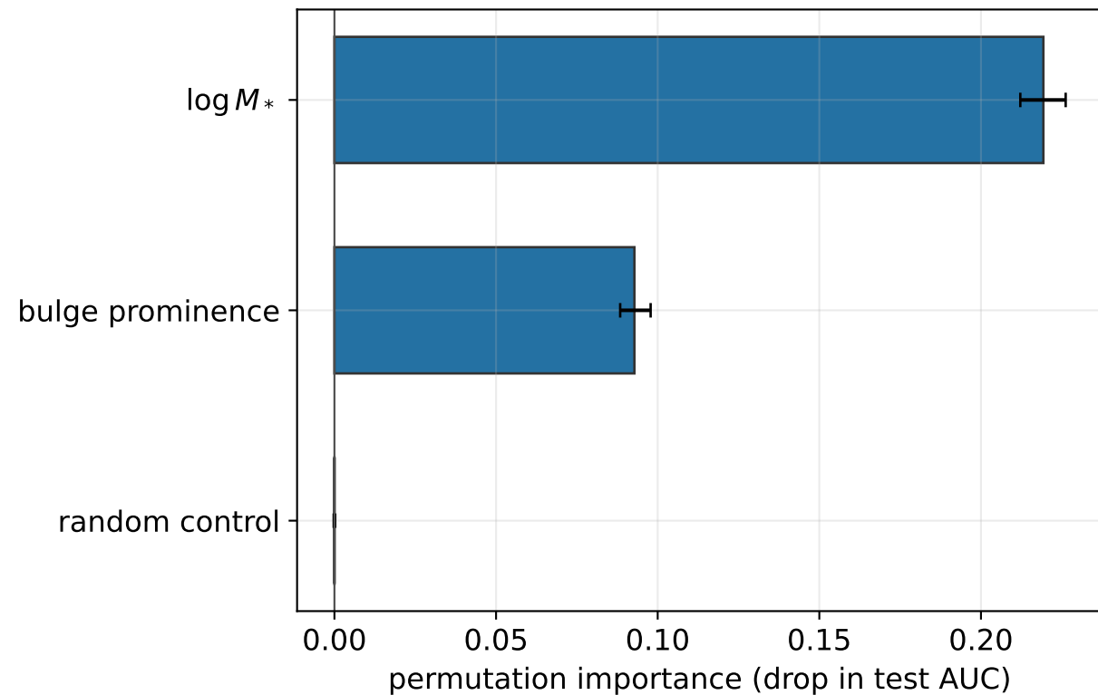
MAIN: within-disc quenching median AUC = 0.862
