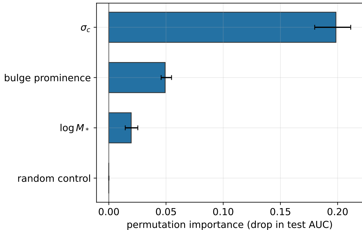
SIGMA-clean: add \sigma_c median AUC = 0.828
