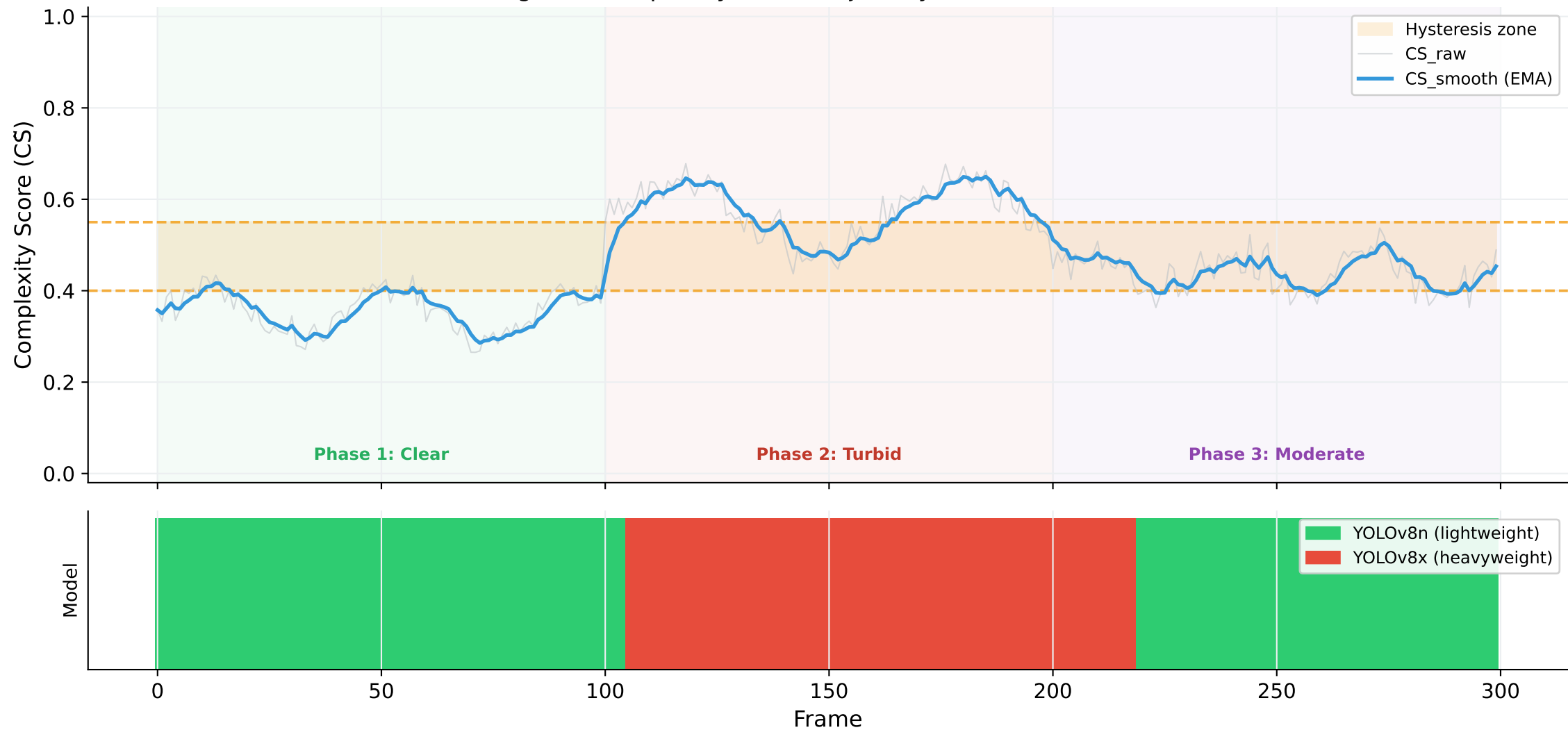
Fig 1 — Complexity Score Trajectory & Model Selection
