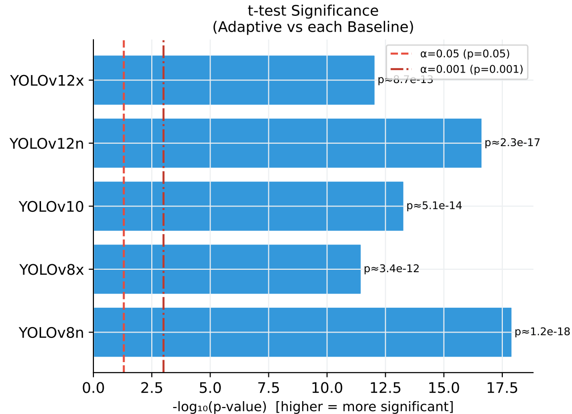
Fig 8 — Statistical Significance Summary
