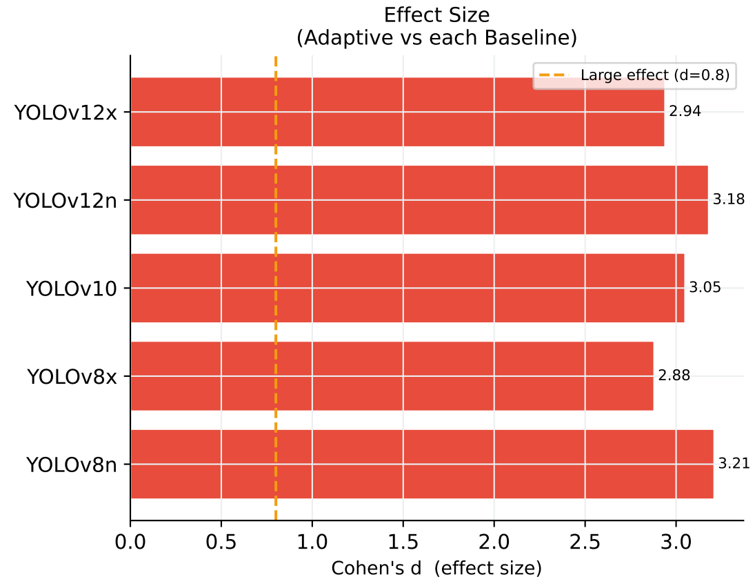
Fig 8 — Statistical Significance Summary
