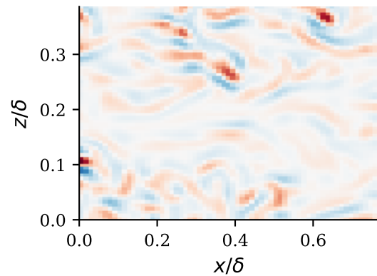
(e) Jaumann hybrid
