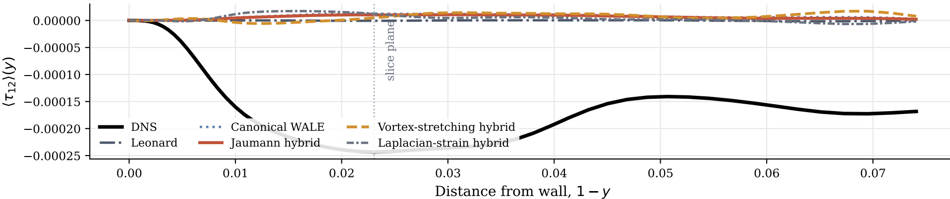
(a) Mean SGS shear profile
