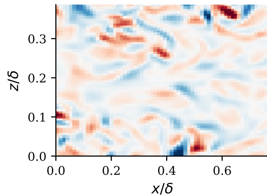
(f) Vortex-stretching hybrid
