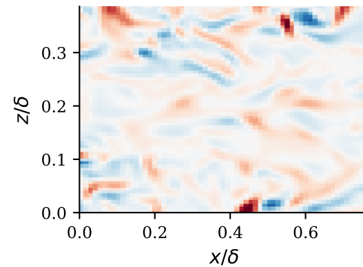
(g) Laplacian-strain hybrid
