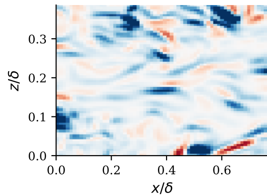
(b) DNS
