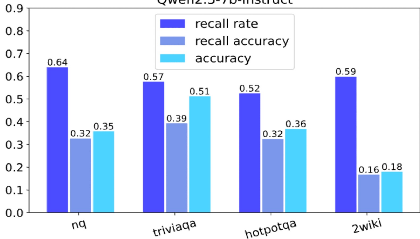
Qwen2.5-7b-Instruct
