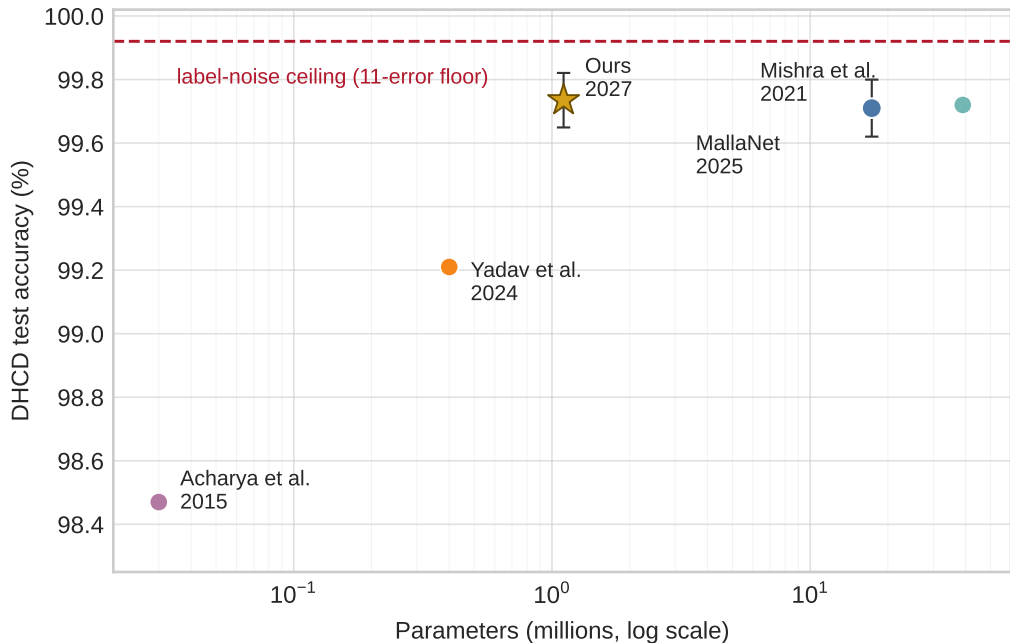
Accuracy vs. Parameters on DHCD
