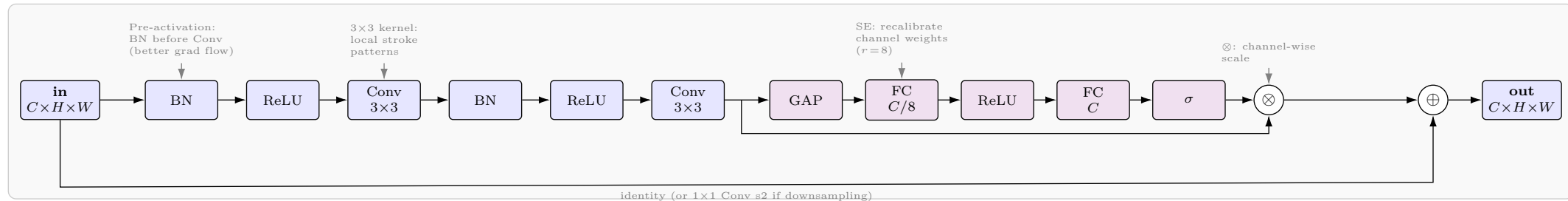
(b) PreAct SE-ResBlock (unravelled)
