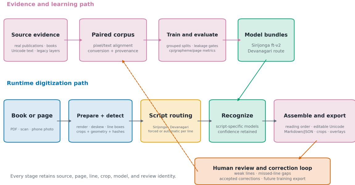
Figure 1: LimbuOCR system architecture. The upper path constructs and validates evidence and model bundles; the lower path performs page-to-book OCR. Review decisions remain attached to source crops and can feed later audited training exports.
