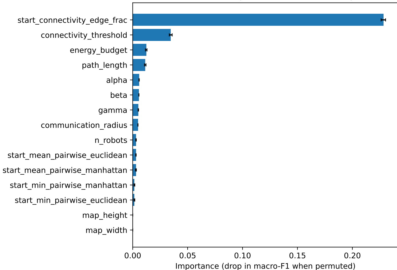
Router Feature Importance (ACO vs SA, top 15)
