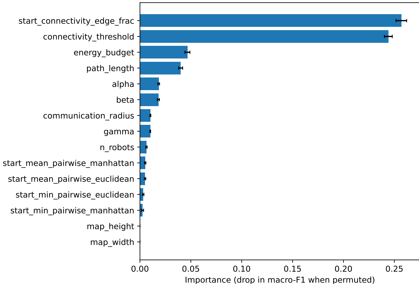
Router Feature Importance (multiclass, top 15)
