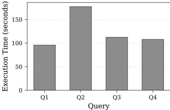
Execution Time - Abacus
