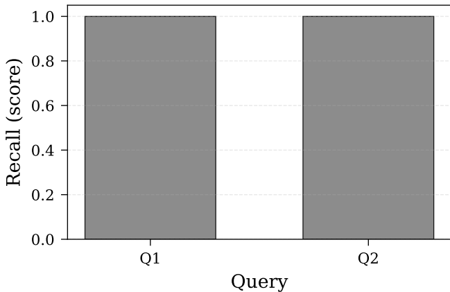
Recall - Abacus
