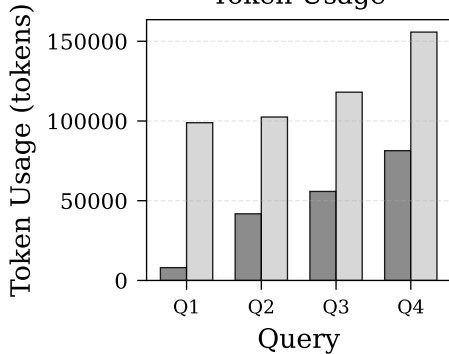
Token Usage
