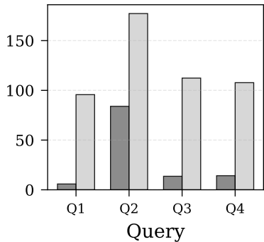
Execution Time
