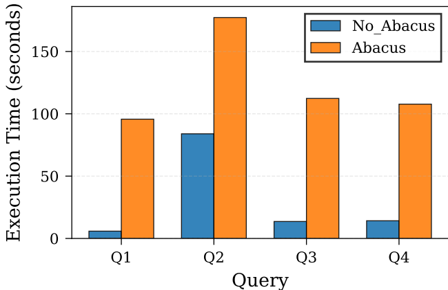
Execution Time Comparison
