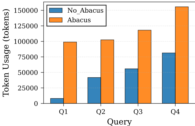
Token Usage Comparison
