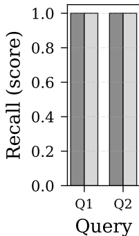
Recall
