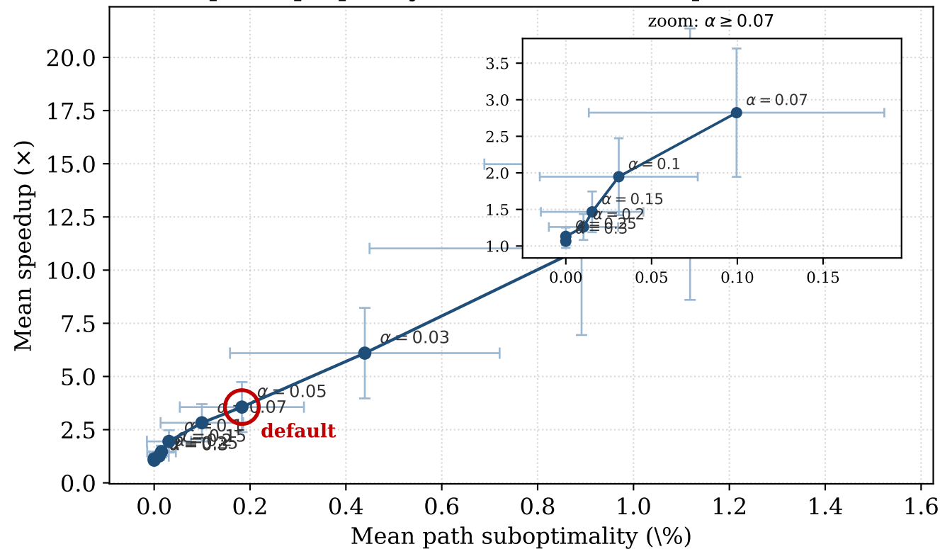
Speedup--quality Pareto frontier (Experiment 7)
