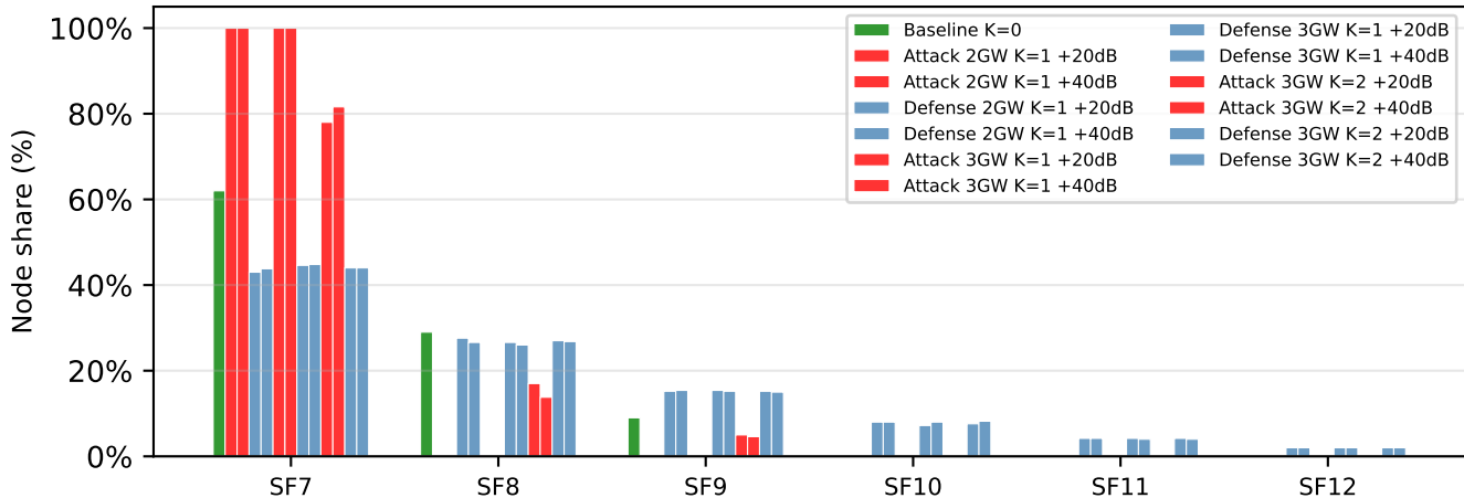
Final Spreading Factor Distribution
